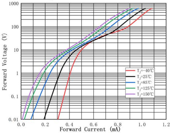
Fig. 3: Forward Characteristics
